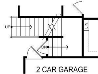
STAIRS TO OPT BASEMENT
