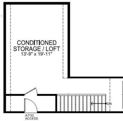
OPT CONDITIONED STORAGE / LOFT
