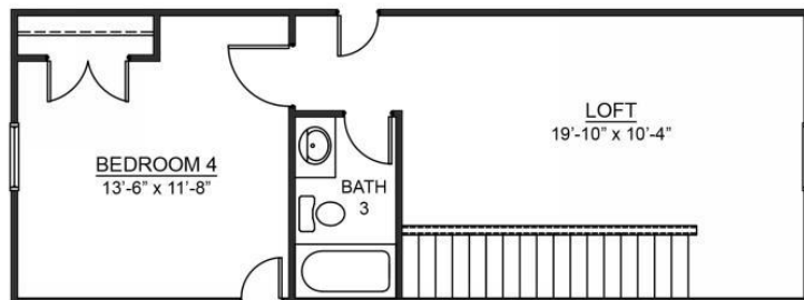
OPT. SECOND FLOOR
